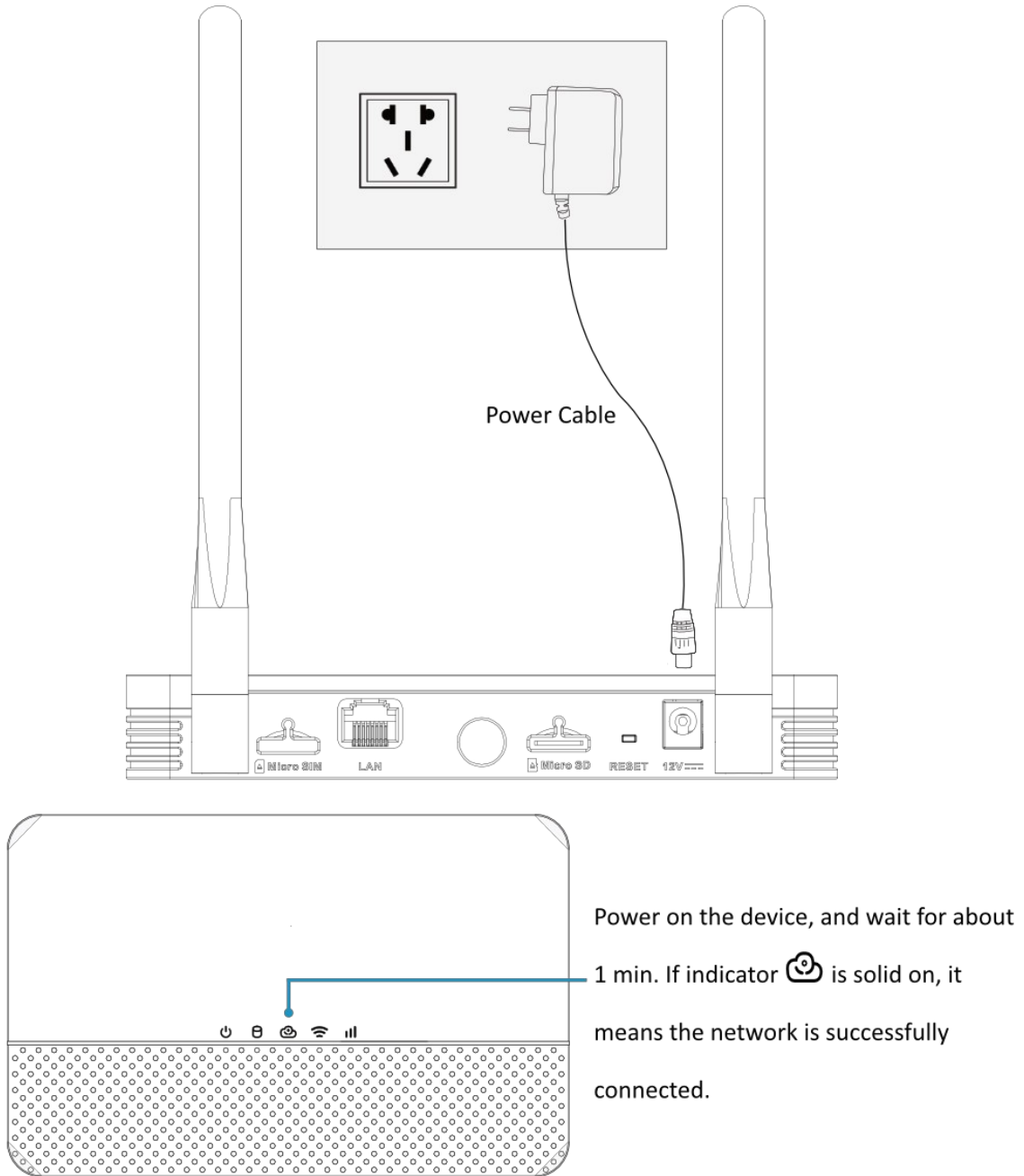
Figure 4-1 Startup
